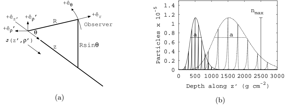
Figure 1: (a) Coordinate systems. Un-primed coordinates refer to the observer, and primed coordinates refer to the reference frame of the vector current. (b) The curves represent the total charge content, with the instantaneous charge density (ICD) shown by the internal curves, versus depth after the first interaction in the medium. The solid curves were made for shower energy 10^{14} eV and the dashed curves for a shower profile having been stretched by either the LPM effect, or simply by going to a higher energy. The Greisen model was used for the form of the cascade profile. The n_{\text{max}} parameter will refer to the negative charge excess.
