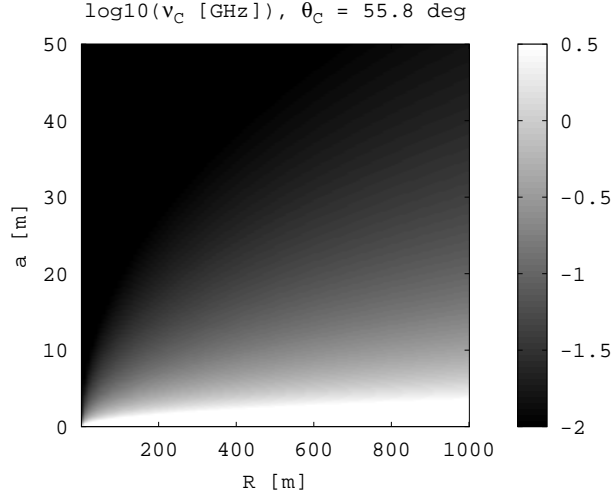
Figure 9: A contour graph of \log_{10} \nu_C , for a parameter space relevant for ground-based radio-Askaryan detectors. Notice that \nu_C < 1 GHz if a \gtrsim 1 m.
