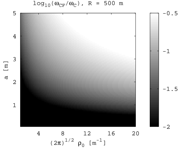
Figure 10: A contour plot of \omega_{CF}/\omega_C = \nu_{CF}/\nu_C , for a parameter space relevant for ground-based radio-Askaryan detectors.
