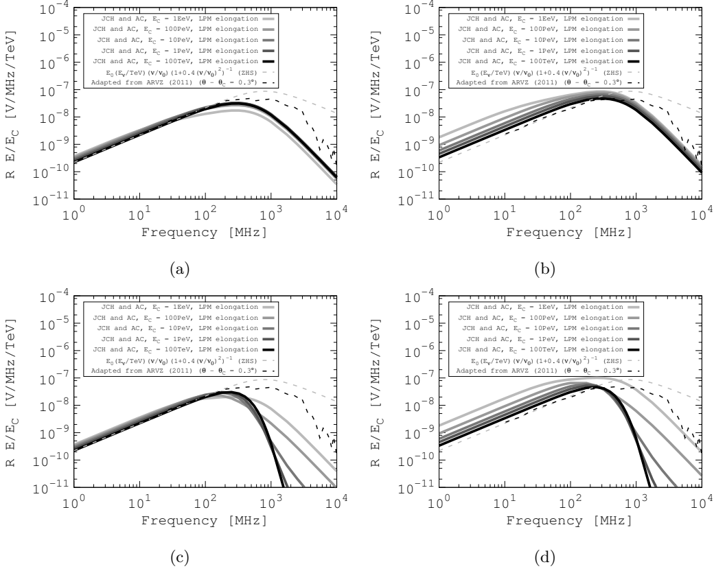
Figure 7: The influence of LPM elongation on |\hat{e}_\theta \cdot \tilde{\mathbf{E}}(\omega)| , for different values of \eta . (a) |\hat{e}_\theta \cdot \tilde{\mathbf{E}}(\omega)| , for R = 200 m, and \theta = 57^\circ , low-frequency restricted. (b) |\hat{e}_\theta \cdot \tilde{\mathbf{E}}(\omega)| , for R = 200 m, and \theta = 57^\circ . (c) |\hat{e}_\theta \cdot \tilde{\mathbf{E}}(\omega)| , for R = 1000 m, and \theta = 57^\circ , low-frequency restricted. (d) |\hat{e}_\theta \cdot \tilde{\mathbf{E}}(\omega)| , for R = 1000 m, and \theta = 57^\circ . In all graphs, the black dashed line is the ZHS result with no LPM elongation, and the gray dashed line is the ARVZ result adapted from Fig. 3 of [32]. See text for detail.
