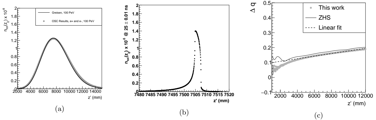
Figure 13: (a) n_{\text{tot}} versus z' , for a 100 PeV cascade. (b) The ICD at 25 \pm 0.01 ns after the first interaction. (c) The fractional negative charge excess of a 100 PeV shower, with a 5 MeV MC threshold from Geant4. The solid line is the ZHS result with a 5 MeV MC threshold, and the dashed line is a linear fit to the OSC results.
