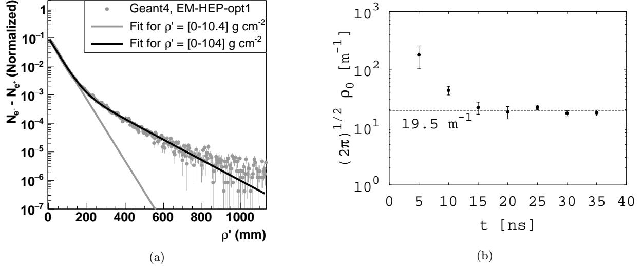
Figure 11: (a) N_{e^-} - N_{e^+} , versus \rho' at 25 ns into a 100 PeV shower (gray points). A single-exponential model (gray line, Eq. 21) with slope \sqrt{2\pi}\rho_0 is fit for \rho' < 10.4 \text{ g cm}^{-2} . A double-exponential model (black line, Eq. 28) is fit for \rho' < 104 \text{ g cm}^{-2} . (b) Fit results for the parameter \sqrt{2\pi}\rho_0 vs. time within the shower, using Eq. 21. The dashed line is the average of the points between 15-35 ns.
