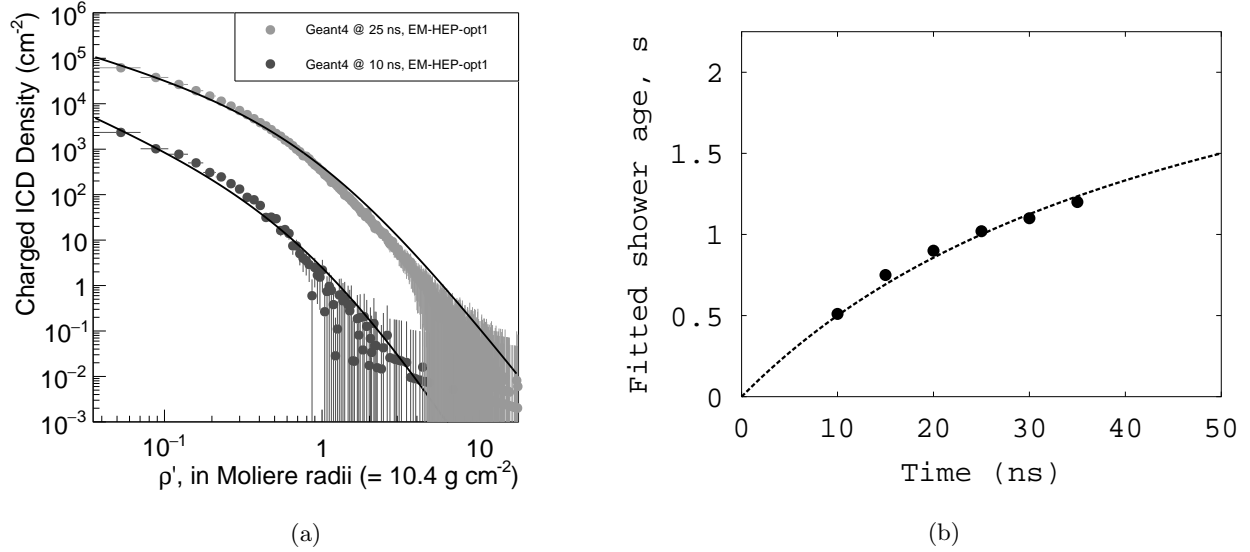
Figure 12: (a) The charged ICD density, at 10 ns and 25 ns after the first interaction. The solid lines are fits of Equation 19 to the points with the shower age, s , as free parameter. (b) The fitted shower age, s , versus time since first interaction. The dashed line is the theoretical expectation.
