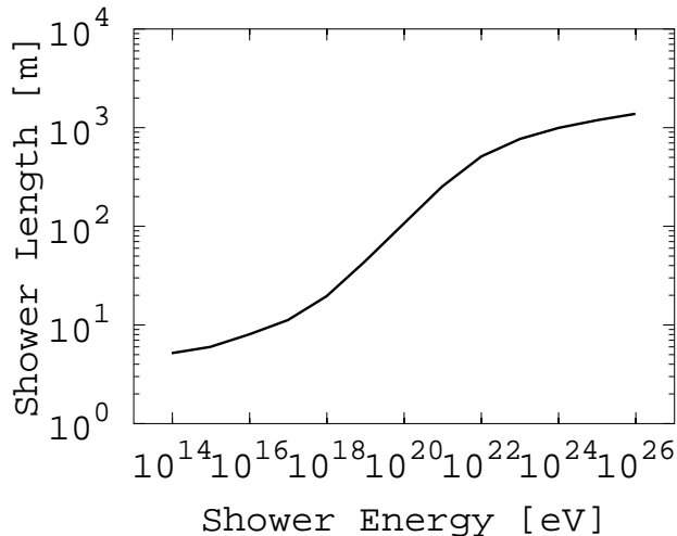
Figure 2: The length of the neutrino-induced cascade, including the LPM effect, from ref. [42].
