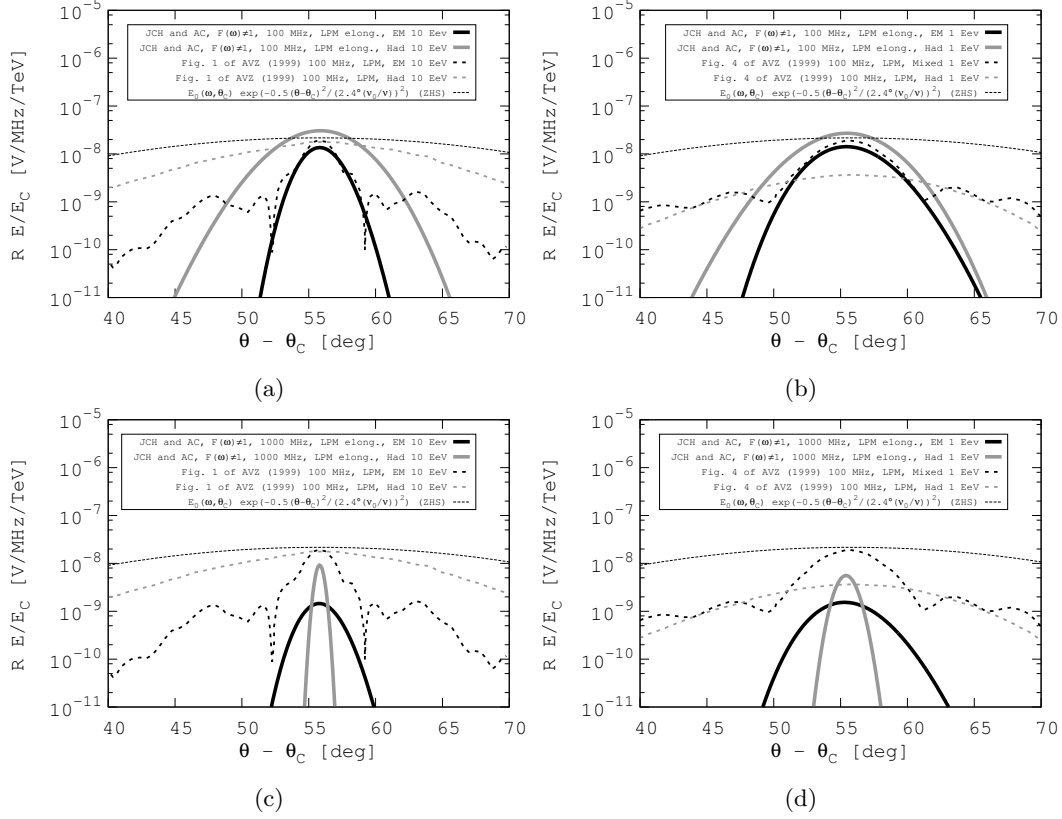
Figure 8: (a) |\hat{e}_\theta \cdot \tilde{\mathbf{E}}(\omega)| versus \theta , for \nu = 100 MHz, E_C = 10 EeV, and R = 2000 m, accounting for LPM elongation, in the pure electromagnetic (solid black) and pure hadronic (solid gray) cases. Shown for comparison are the pure electromagnetic (dashed black) and pure hadronic (dashed gray) from Fig. 1 of [31]. (b) |\hat{e}_\theta \cdot \tilde{\mathbf{E}}(\omega)| versus \theta , for \nu = 100 MHz, E_C = 1 EeV, and R = 500 m, accounting for LPM elongation, in the pure electromagnetic (solid black) and pure hadronic (solid gray) cases. Shown for comparison are the mixed (dashed black) and pure hadronic (dashed gray) from Fig. 4 of [31]. (c) Same as (a), but with \nu = 1000 MHz. (d) Same as (b), but with \nu = 1000 MHz. Notice that for \nu = 1000 MHz, the electromagnetic cone-width is larger than the hadronic cone-width. See text for details.
